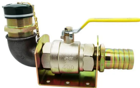
Remote Offset Fill Point - 2" Hose Tail
