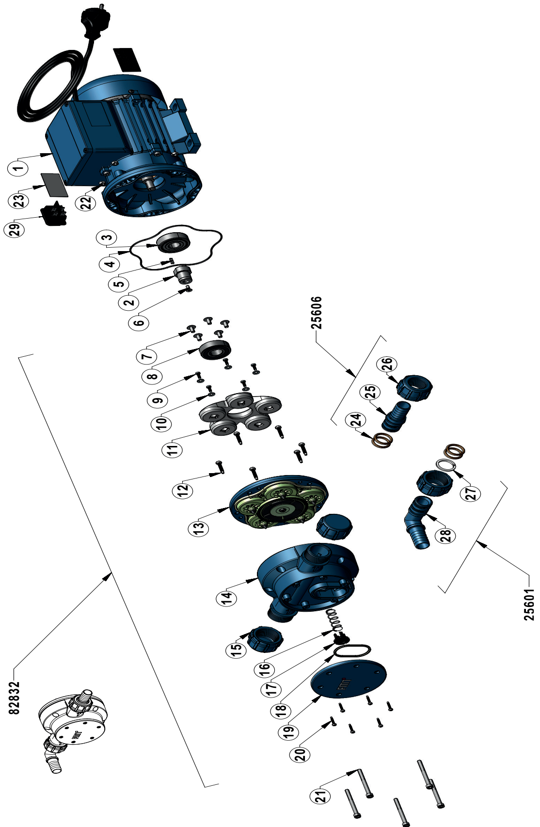
Fig. 15.-1: Exploded view of AdBlue® electric diaphragm pump
